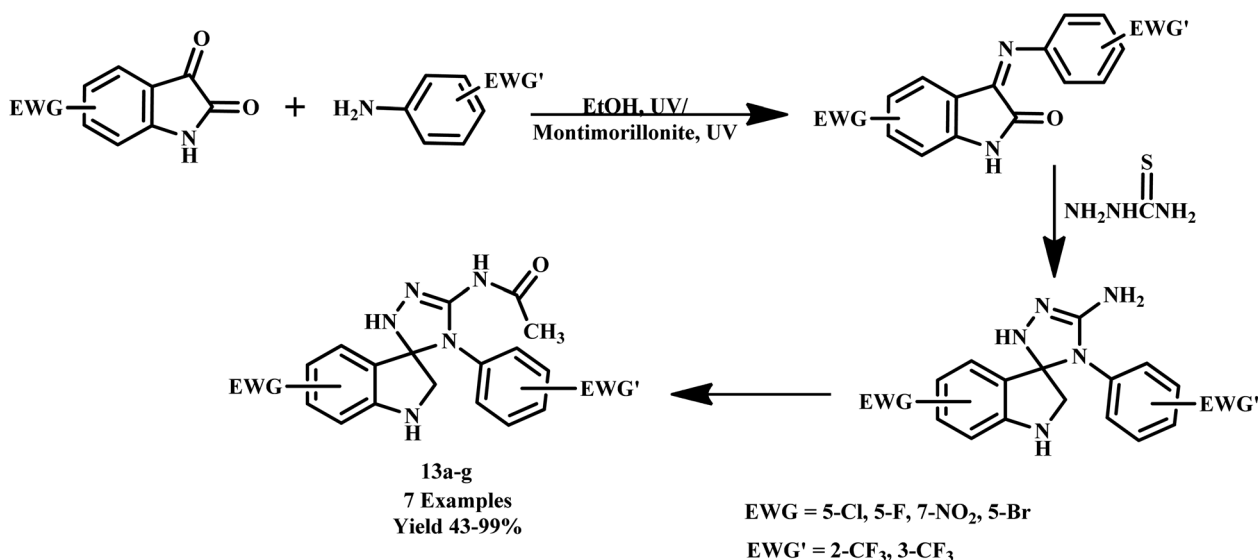
Scheme 8 Synthesis of tri fluoromethyl-substituted spiro[3H-indole-3,3'-[3H-1,2,4]triazole-2(1H)-ones ( 13a–g ). 43
