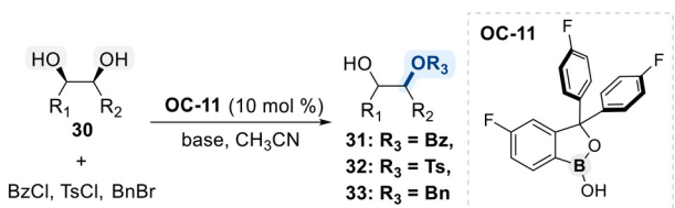
Scheme 19 Chiral benzazaborole-catalyzed enantioselective sulfonation of meso -1,2-diol.
