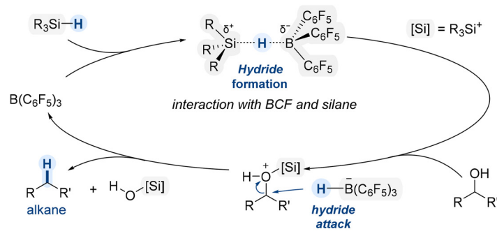
Scheme 2 General mechanism for BCF-catalysed deoxygenation of alcohols.
