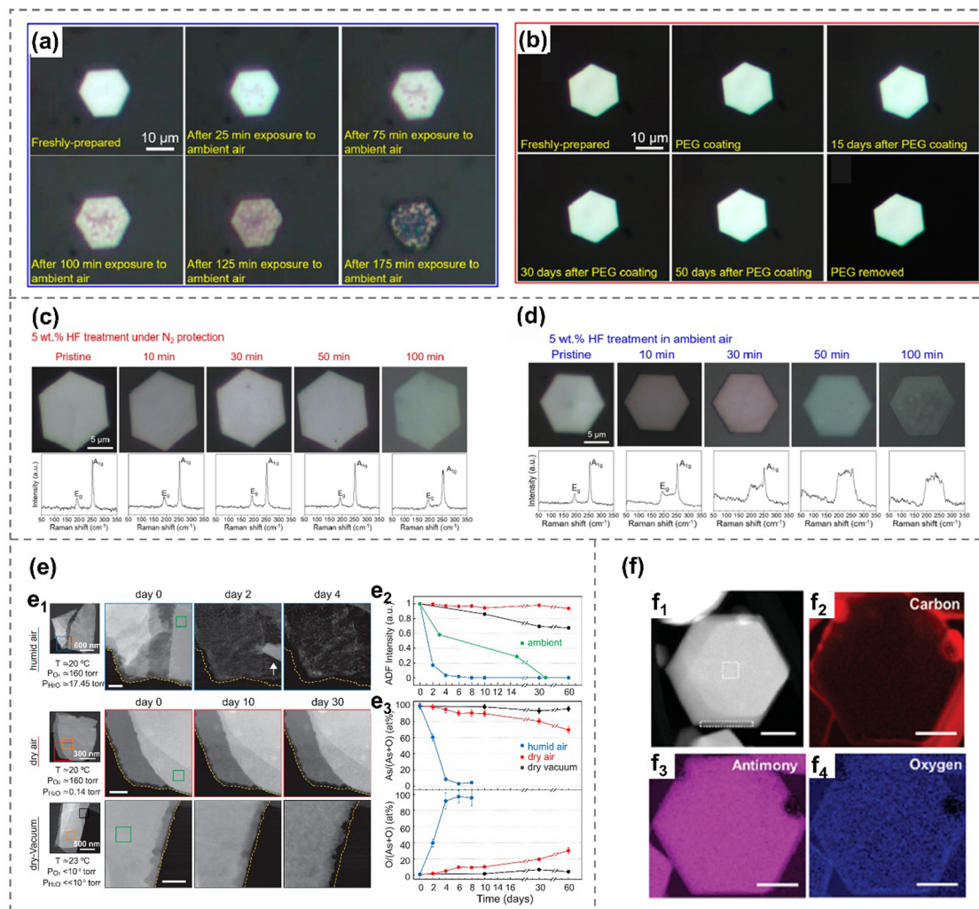
Fig. 5 Oxidation and degradation behavior of arsenene and antimonene. (a) Optical images of a \beta -arsenic nanoflake with varying durations of exposure to the ambient environment. 32 (b) An as-prepared \beta -arsenene nanoflake, followed by its state after PEG coating and removal. 32 (c) and (d) Optical images and corresponding Raman spectroscopy of \beta -arsenene nanoflake after different durations of HF treatment under N_2 protection (b) and in ambient air (c), respectively. 40 (e) Degradation of exfoliated \alpha -arsenene flakes under humid air, dry air and dry-vacuum environment. 38 HADDF-STEM images showing degradation of \alpha -arsenene over time ( e_1 ). Changes in HAADF intensity of \alpha -arsenene with time ( e_2 ). Elemental composition of \alpha -arsenene over time measured by EDX ( e_3 ). (f) HADDF-STEM image ( f_1 ) and elemental compositional EELS maps ( f_2 )–( f_4 ) of few-layer antimonene hexagons. 106 Reproduced from: (a), (b) ref. 32 with permission from American Chemistry Society, Copyright 2019; (c), (d), ref. 40 with permission from Wiley-VCH, Copyright 2021; (e) ref. 38 with permission from American Chemistry Society, Copyright 2020; (f) ref. 106 with permission from Wiley-VCH, Copyright 2021.
