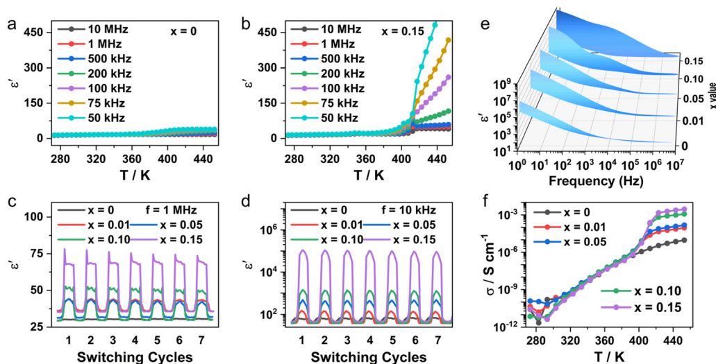
Fig. 4 [\text{C}_5\text{H}_{12}\text{N}]_{2-2x}\text{Pb}_{1-x}\text{Mn}_x\text{Cl}_{4-2x} : plots of \epsilon' vs. T at selected AC frequencies for x = 0 (a) and x = 0.15 (b). Dielectric switching responses for x = 0-0.15 at AC frequencies of 1 MHz (c) and 10 kHz (d). Frequency dependence of the DSR in the 383–433 K range for x = 0-0.15 (e). Plots of \sigma vs. T for x = 0-0.15 (f).
