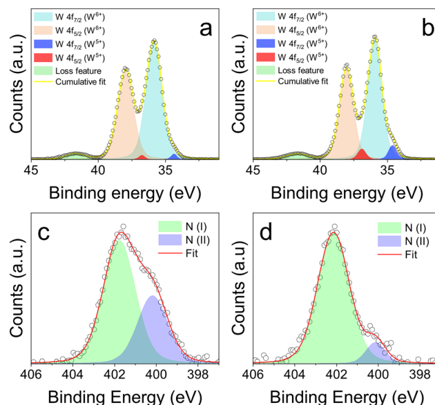
Fig. 2 (a and b) XPS spectra of the W 4f region of undoped (a) and \text{MA}^+ doped (b) \text{WO}_{3-x} NCs. (c and d) XPS spectra in the N 1s region for doped NCs before (c) and after (d) treatment with trifluoroacetic acid.
