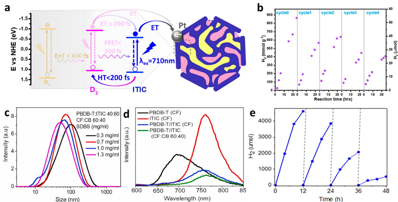
Fig. 24 (a) Scheme of photophysical pathways of D 1 (PFBT)/D 2 (PFODTBT)/ITIC ternary BHJ PCs. (b) Recycling experiment of hydrogen evolution. A 35 mg amount of ascorbic acid was added after cycle 1 and cycle 3, and the final pH was adjusted to pH 4 with 2 M KOH solution. Adapted with permission. 97 Copyright 2021, American Chemical Society. (c) Size distribution of BHJ (PBDB-T:ITIC) nanoparticles with varied SDBS concentration. (d) PL spectra excited at 520 nm of PBDB-T, ITIC, and BHJ nanoparticles fabricated using single solvent (CF) and binary solvent mixture (CF/CB). (e) The stability test of the BHJ nanoparticles during a long-term photocatalytic hydrogen production. Adapted with permission. 98 Copyright 2022, Elsevier. Ltd.
