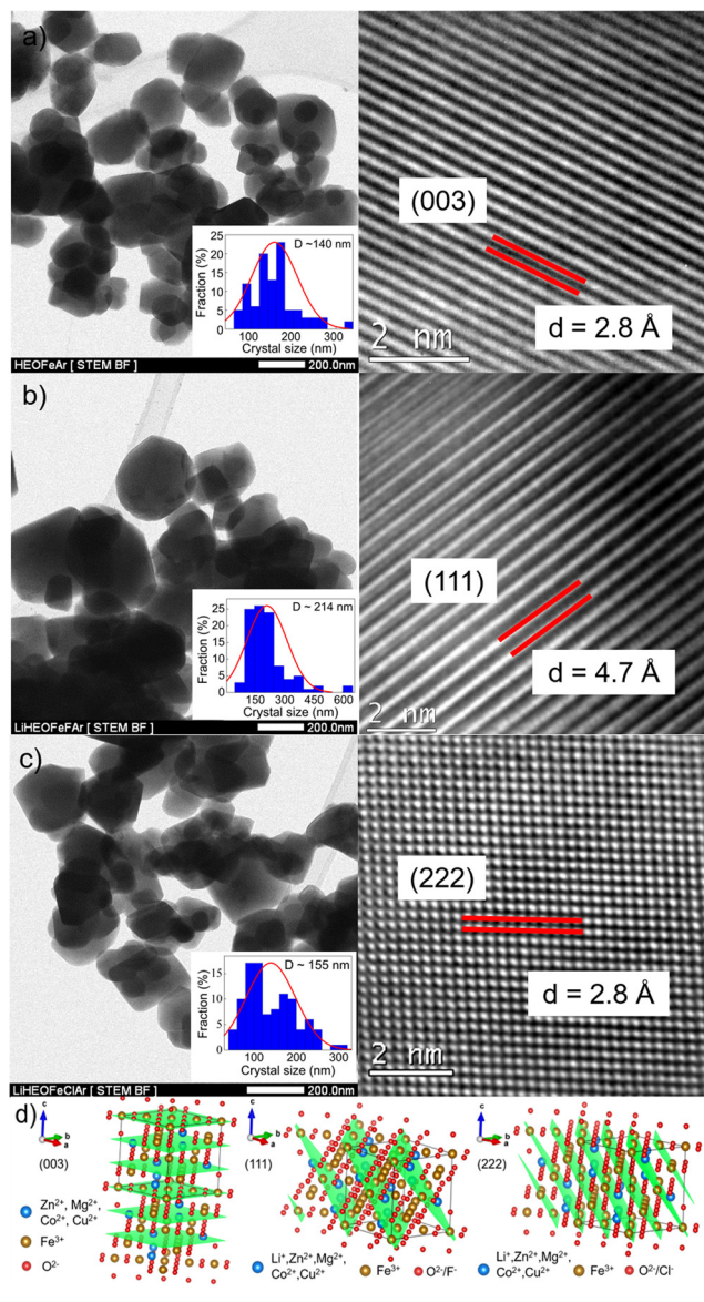
Fig. 2 (S)TEM and HR-TEM micrographs of (a) HEOFe, (b) LiHEOFef, and (c) LiHEOFecI synthesized samples. Insets show the particle size distribution. Interplanar distances, d , correspond to those determined from eqn (5). (d) Idealized spinel structure of the investigated samples. Particular crystal planes for HEOFe (003), LiHEOFef (111), and LiHEOFecI (222) are highlighted.
