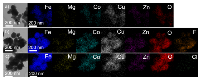
Fig. 3 (S)TEM micrograph of the synthesized (a) HEOFe, (b) LiHEOFef, and (c) LiHEOFecI samples with the corresponding elemental maps determined by EDS.
