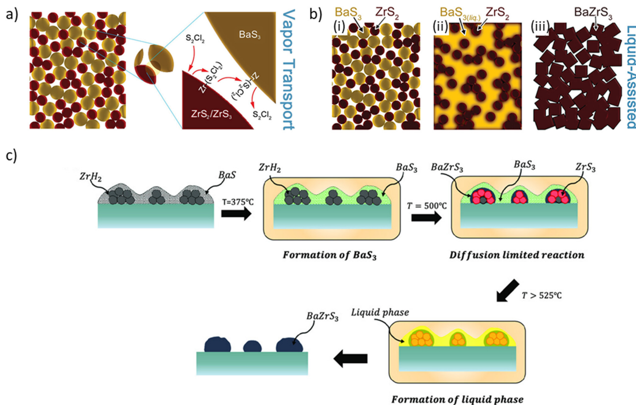
Fig. 10 Schematic illustrating the working principles of: (a) \text{S}_2\text{Cl}_2 vapor transport agent, (b) \text{BaS}_3 liquid flux, and (c) \text{BaS}_x ( x > 3 ) liquid flux. (a) Reproduced with permission. 100 Copyright 2023, American Chemical Society. (b) Reproduced with permission. 101 Copyright 2023, Wiley.
