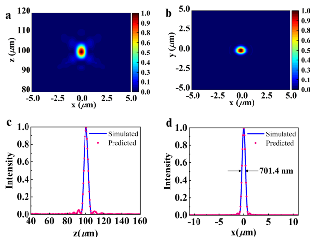
Fig. 11 Intensity profile of \text{TiO}_2 based metalens (a) in the ( x - z ) plane and (b) in the ( x - y ) plane) of the focal spot in the focal plane. (c) Normalized intensity distribution (simulated and predicted) at the focal point along the propagation direction ( z -axis). (d) Corresponding horizontal cut at the focal spot in (b). Here, the FWHM of the focal spot is 701.4 nm.
