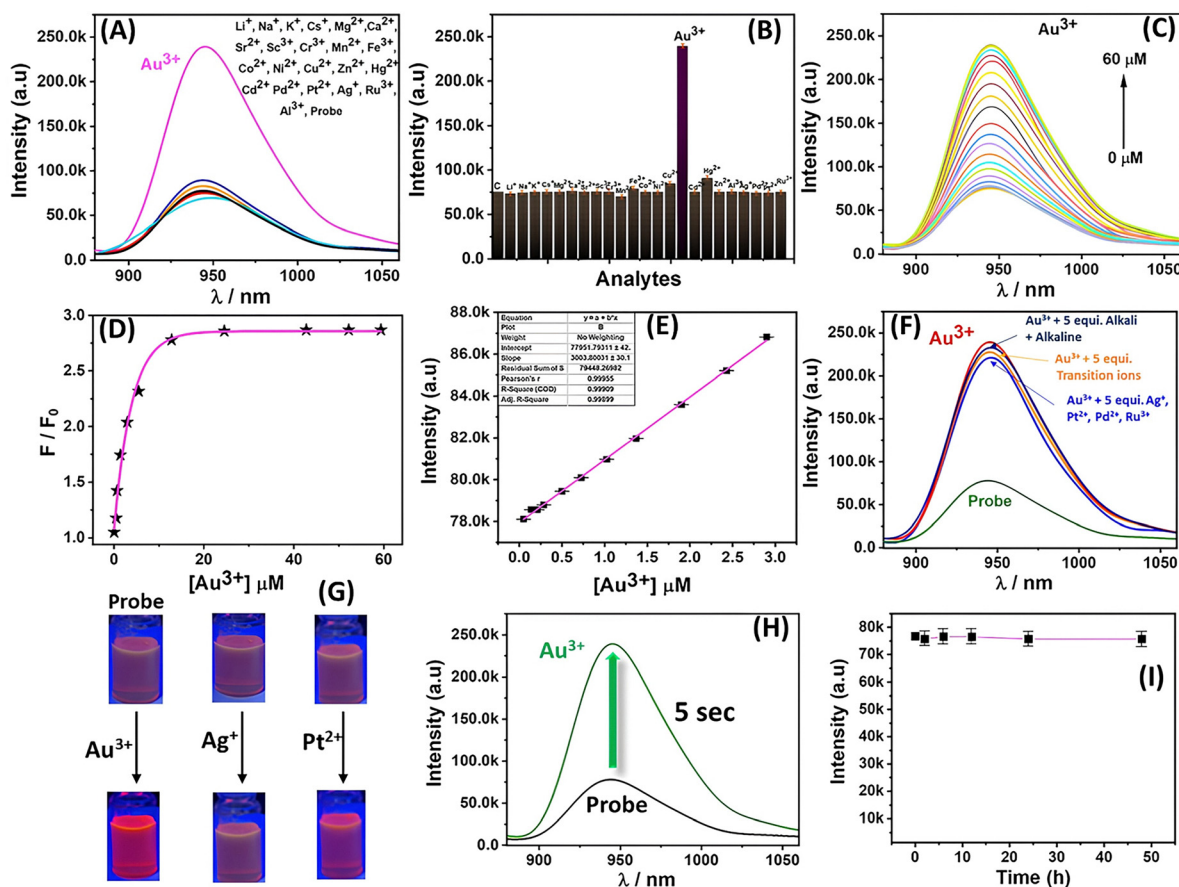
Fig. 3 (A) The fluorescence selectivity screening with various ions. (B) The relative fluorescence emission intensity of the material with different cations. (C) The titration profile with the Au^{3+} ions. (D) The non-linear binding plot with Au^{3+} ions. (E) The LOD (limit of detection) plot. (F) The interference study plot of the material with an excess of alkali, alkaline, transition, and precious metal ions. (G) The pictures of the probe material (long-wave UV; 365 nm) before and after the addition of Au^{3+} , Ag^+ , and Pt^{2+} ions. (H) The fast response behaviour of the material toward Au^{3+} ions. (I) The plot fluorescence emission stability with respect to time.
