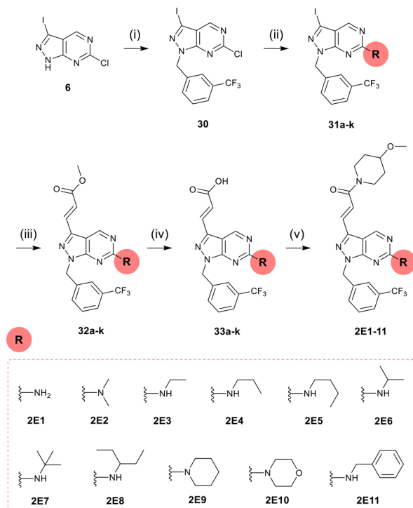
Scheme 5 Synthesis of 2E1–11 . Reagents and conditions: (i) 3-(trifluoromethyl)benzyl alcohol, DIAD, PPh 3 , THF, under N 2 , r.t., 50%; (ii) appropriate amine (R), THF, 150 °C, \mu w, 60 min; (iii) methyl acrylate, Pd(OAc) 2 , PPh 3 , TEA/dioxane, under N 2 , 100 °C, 24 h, 79–97%; (iv) aqueous NaOH, THF, 60 °C, 24 h; (v) 4-methoxypiperidine, DIPEA, HATU, DMF, r.t., 2 h, 30–87%.
