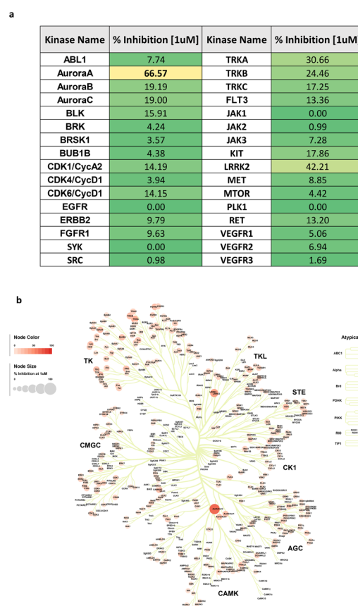
Fig. 9 Kinase inhibition profile of lead 2D7 . a ) Summary of kinase profiling. Table shows the percentage of enzymatic inhibition after treatment with 1 \mu\text{M} of 2D7 , the mean percentage are respect to DMSO control. Colour scale highlights the inhibition percentage values from the lowest (green) to the highest (red). b ) Kinome phylogenetic tree showing the selectivity of compound 2D7 for the Aurora kinase A over a panel 340 protein kinases. Note that only kinases listed on Coral software 44 were used for this plot. The size of the dots is relative to the mean percentage (%) of inhibition to the corresponding kinase at a dose of 1 \mu\text{M} . Where dots are not present, the kinase was not evaluated.
