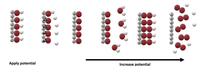
Fig. 7 OER mechanism as described by Rossmeisl and Nørskov. 46 Silver: metal surface; red: oxygen; white: hydrogen. When a potential is applied, water molecules dissociate and form \text{OH}_{\text{ad}} (eqn (13)). Without a further increase in potential, a proton is split off into solution and an electron to the electrode (eqn (14)). After this, the coverage of \text{O}_{\text{ad}} increases until no new \text{OH}_{\text{ad}} forms. If the potential is high enough, water molecules will adsorb on \text{O}_{\text{ad}} , forming \text{OOH}_{\text{ad}} (eqn (15)) and eventually evolve \text{O}_2 (eqn (16)).
