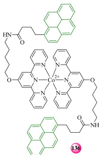
Fig. 42 Bis(4-pyren-1-yl- N -[5-[(2,2';6',2'')]terpyridin-4'-yloxy]-pentyl]-butyramide)cobalt(II) ion ( [\text{Co}(\text{tpy} \sim \text{py})_2]^{2+} ), complex 136 . Reproduced with permission from ref. 58 copyright 2009, American Chemical Society.
