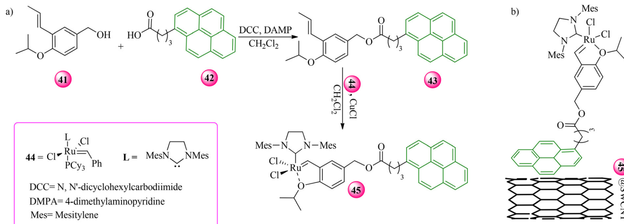
Fig. 17 The scheme of (a) the synthesis procedure for the pyrene-tagged ruthenium complex ( 45 ) and (b) immobilization of ( 45 ) on the SWCNT surface. Reproduced with permission from ref. 13 copyright 2009, American Chemical Society.
