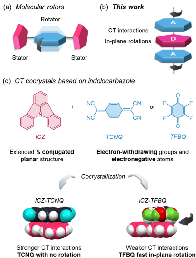
Fig. 1 Schematic illustration of motion (a) in a molecular rotor and (b) in this work. (c) The design of the new CT cococrystals is reported here, with the molecular motion in one instance.
