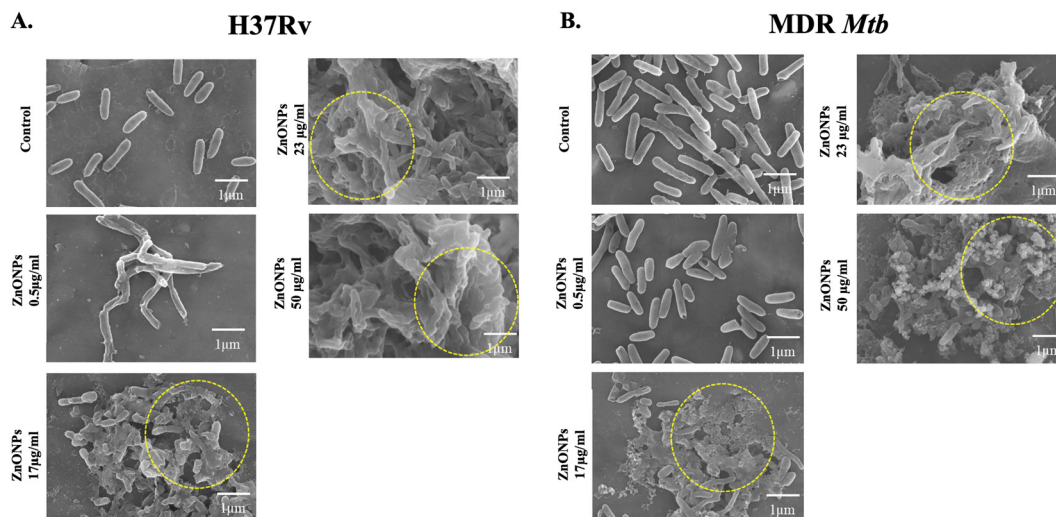
Fig. 5 SEM analysis displaying the bactericidal effect of ZnONPs on Mycobacterium tuberculosis (Mtb) cells: (A) H37Rv and (B) MDR Mtb isolates. Control (untreated) mycobacterial cells were uniform looking, without any changes in the cell morphology or any evidence of membrane damage. Mild alterations in cellular morphology were noted for both H37Rv and MDR Mtb cells in the presence of 0.5 µg ml -1 ZnONPs. Dose dependent increase in the severity of cell membrane damage, cell fusion, and loss of cellular architecture were identified among the (A) H37Rv and (B) MDR Mtb isolates, across the rest of the ZnONP test concentration ranges (17 µg ml -1 , 23 µg ml -1 , and 50 µg ml -1 ) (outlined by yellow circles). MDR: multidrug-resistant Mtb.
