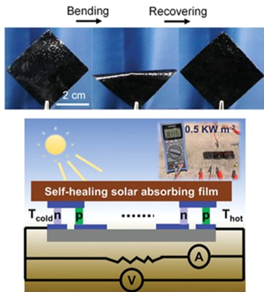
Fig. 10 Illustration of the excellent flexibility of the H-PDMS/CR43 film (top) and schematic illustration of the STEAG device (bottom). Reproduced with permission from ref. 6. Copyright 2022, Wiley.
