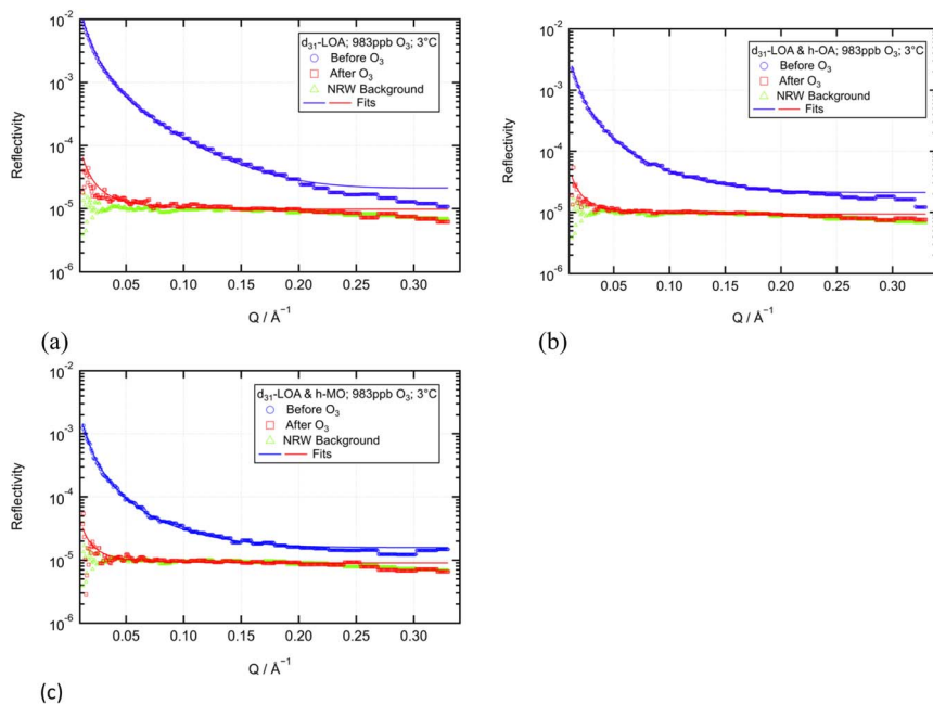
Fig. 10 R vs. Q reflectivity plots before and after reaction with O_3 of (a) a pure d-LOA monolayer (21 \mu\text{L} of 1.4 \text{ g L}^{-1} d-LOA; [O_3] = 983 \pm 150 \text{ ppb} ; 3 \pm 1^\circ\text{C} ); (b) d-LOA in a mixed monolayer with h-OA (21 \mu\text{L} of 0.68 \text{ g L}^{-1} d-LOA/ 0.75 \text{ g L}^{-1} h-OA; [O_3] = 983 \pm 150 \text{ ppb} ; 3 \pm 1^\circ\text{C} ); and (c) d-LOA in a mixed monolayer with h-MO (21 \mu\text{L} of 0.65 \text{ g L}^{-1} d-LOA/ 1.0 \text{ g L}^{-1} h-MO; [O_3] = 983 \pm 150 \text{ ppb} ; 3 \pm 1^\circ\text{C} ). Null-reflecting water (NRW) backgrounds are shown for comparison.
