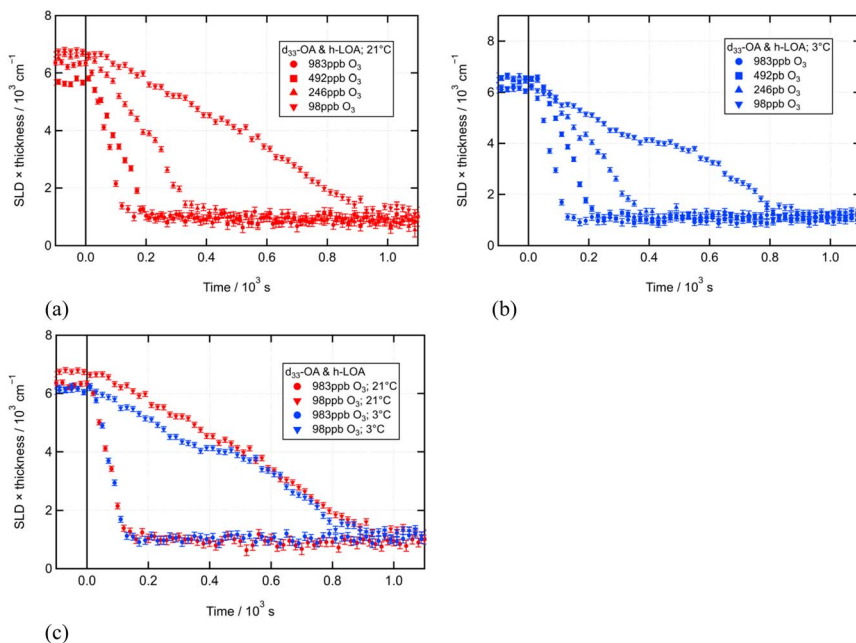
Fig. 2 Time evolution of fitted neutron reflectometry signal during oxidation of d-OA in a mixed monolayer with h-LOA (21 \mu L of 0.81 g L -1 d-OA/0.59 g L -1 h-LOA; O 3 introduced at t = 0 s at various [O 3 ]) at (a) room temperature (21 \pm 1 °C) and (b) near-freezing (3 \pm 1 °C). (c) Re-plots the data for the highest and lowest ozone concentrations to compare directly the behaviour at the two different temperatures.
