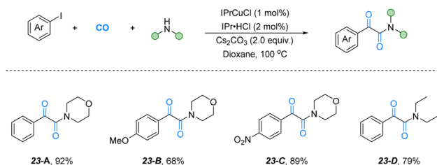
Fig. 23 Copper-catalyzed double carbonylation of aryl iodides and amines.
