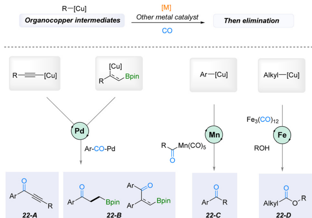
Fig. 22 Transmetalation of organocopper intermediates into other metal catalysts.
