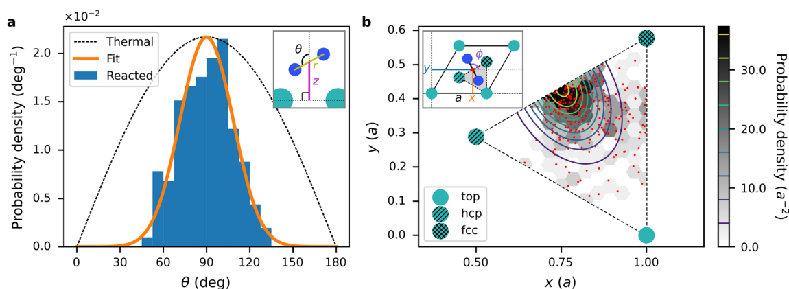
Fig. 4 Distributions for initial (a) orientation \theta and (b) xy position of N 2 molecules above the Ru(0001) surface for E_{\text{inc}} = 3.25 eV ( > E_{\text{a}}^{\text{TS}} = 1.83 eV) and \nu = 0 . The coordinates are depicted in the insets. (a) The initial distribution for all trajectories (both reacted and non-reacted, black dashed line, eqn (S6) in the ESI†) is compared to the distribution of the subset comprised by the reacted trajectories (blue bars). To guide the eye, the latter has been fitted to the initial distribution multiplied by a Gaussian centred at \theta = 90^\circ (orange line, eqn (S7) in the ESI†). (b) The distribution for the initial xy -position of reacted trajectories in the irreducible wedge of the unit cell, as depicted in the inset. a denotes the surface lattice constant. Individual reacted trajectories are in red, the histogram is in greyscale, and the fitted bimodal Gaussian distribution is the contour lines. For better comparison and to quantify dynamical steering effects, the reacted distributions have been rescaled such that their maxima coincide with those of the distributions for all trajectories.
