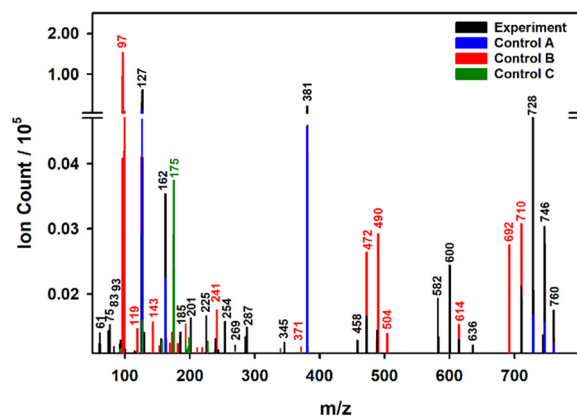
Fig. 5 ESI-MS analysis after 10 min irradiation ( \lambda_{\text{cut-off}} \geq 295 nm) at pH 7.0 for the following conditions: (black) experiment with 30 \mu M iohecol, 3.0 mg L -1 humic acids, and 5.5 mg L -1 ClO - ; (blue) control A, lacking humic acids; (red) control B, lacking ClO - ; and (green) control C, lacking iohecol. Each spectrum represents the difference between the 10 min and corresponding 0 min time points. Labeled m/z values are color-coded to match the spectrum in which they appear with the highest intensity.
