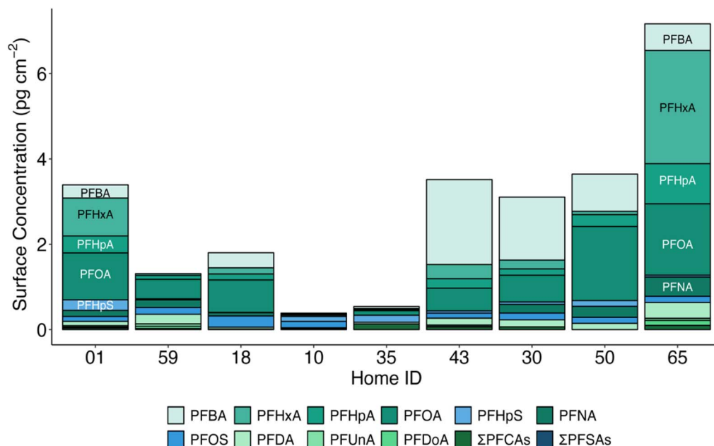
Fig. 3 6 month glass slab PFAA profiles. PFCAs are shades of green and PFASs are shades of blue. PFAS with DF > 50% are shown individually and those with lower DFs as \Sigma PFCA or \Sigma PFAS. PAPs are shown in Fig. S2.† Note that no GS were mounted in home 78.
