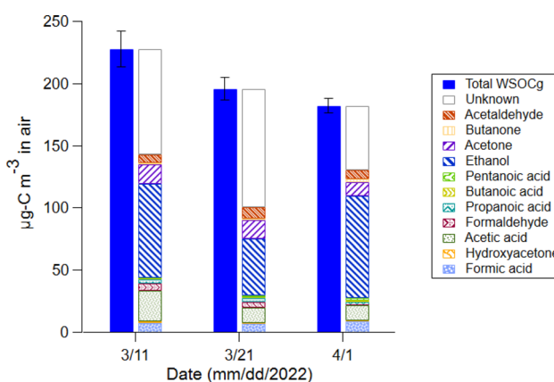
Fig. 2 WSOC g (blue bar) measured with the MC with TOC analyzer and reconstructed WSOC g (multicolored stack) which was taken to be the sum of carbon in measured individual water-soluble organic gases ( K_H > 13 \text{ M atm}^{-1} ) and the remaining mass of carbon (difference between WSOC g and sum of species; white) from unperturbed periods ( i.e. , the house background) on March 11 th , March 21 st , and April 1 st (see Tables S2 and S3†). Compounds are stacked from most (bottom) to least (top) water soluble. The concentration of total WSOC g was corrected for the effective WSOC g collection efficiency (57%). Error bars represent \pm 1\sigma . "House background periods" refer to time periods immediately before conditions were perturbed by scripted activities (typically 1 h to 2 h before the perturbation), 12 h to 16 h after the last perturbation, and sometimes shortly (1 h to 2 h) after perturbations that did not induce an observable change in WSOC g .
