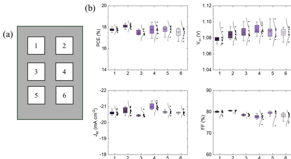
Fig. 5 (a) Bottom plate with the device layout of the six samples. (b) Performance statistics for the devices that have been converted: PCE, V_{\text{oc}} , J_{\text{sc}} , and FF.
