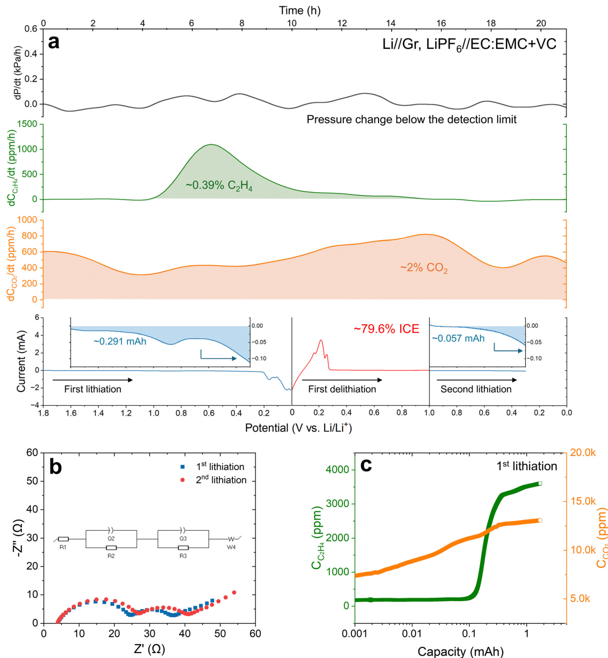
Fig. 7 Operando monitoring of gas evolution in the Li-graphite half-cell that undergoes cyclic voltammetry at a scan rate of 0.05 \text{ mV s}^{-1} with 1 \text{ M LiPF}_6 in \text{EC} : \text{EMC} 3 : 7 \text{ vol\%} + 2 \text{ vol\% VC} as the electrolyte. (a) The obtained CV curves are plotted in conjunction with the change in concentrations of \text{C}_2\text{H}_4 , \text{CO}_2 , and in overall gas pressure. The detailed current variation from 1.8 \text{ V} to 0.3 \text{ V} vs. \text{Li/Li}^+ of the first lithiation and from 1 \text{ V} to 0.3 \text{ V} vs. \text{Li/Li}^+ of the second lithiation is provided in the insets by zooming in the y-axis. The blue shading of the first lithiation represents the electric charge consumed for the SEI formation and associated gas evolution. (b) The EIS spectra obtained after the initial and the second cathodic scan. (c) Evolution of \text{C}_2\text{H}_4 and \text{CO}_2 concentrations during the initial lithiation of graphite.
