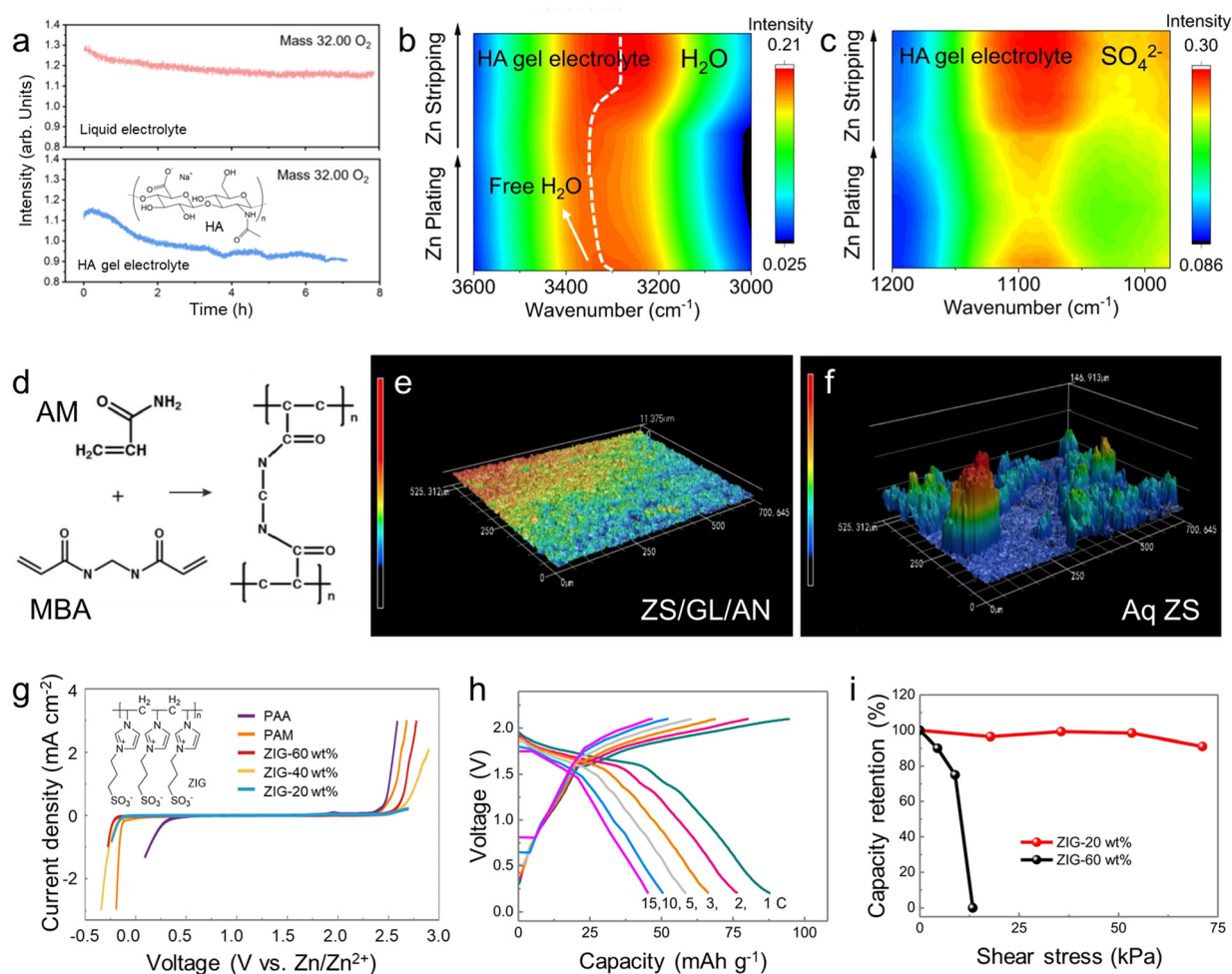
Fig. 5 Design strategies of GPE for high-voltage AZIBs. (a) The \text{O}_2 spectra obtained from differential electrochemical mass spectrometry of \text{Zn}||\text{LMO} cells upon charge/discharge at a current rate of 1C in the liquid electrolyte and the HA gel electrolyte. The inset depicts the chemical structure of HA. In situ synchrotron-FTIR spectra in attenuated total reflection (ATR) mode of stainless-steel electrode during Zn plating/stripping. (b) \nu(\text{OH}) -HA gel electrolyte, (c) \nu(\text{SO}_4^{2-}) -HA gel electrolyte. Reproduced with permission from ref. 115. Copyright 2023, Springer Nature. (d) The polymerization mechanism diagram of the hydrogel electrolyte. The corresponding 3D surface topographies of the cycled Zn electrodes with (e) the hydrogel electrolyte and (f) the conventional electrolyte. Reproduced with permission from ref. 116. Copyright 2022, Elsevier. (g) LSV of ZIG (20, 40, 60 wt% water content), PAM and PAA (conventional HPEs). The inset presents the chemical structure of ZIG. (h) Discharging-charging profiles of \text{Zn}||\text{MnHCF} cell with the ZIG-20 wt% electrolyte at different rates. (i) Capacitance retentions of the full battery based on ZIG with 20 wt% and 60 wt% water contents at different shear stresses. Reproduced with permission from ref. 111. Copyright 2023, Springer Nature.
