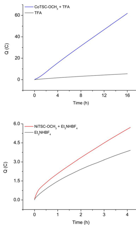
Fig. 2 Coulometry of CoTSC- \text{OCH}_3 with 60 mM TFA during bulk electrolysis experiment at -1.6\text{ V vs. Fc}^{+/0} (top blue line) and blank experiment of 60 mM TFA in the absence of CoTSC- \text{OCH}_3 (top grey line) and NiTSC- \text{OCH}_3 with 100 mM \text{Et}_3\text{NHBF}_4 during bulk electrolysis experiment at -2.1\text{ V vs. Fc}^{+/0} (bottom red line) and blank experiment of 100 mM \text{Et}_3\text{NH}^+ in the absence of NiTSC- \text{OCH}_3 (bottom grey line). The electrolytic solutions contain 0.1 M \text{NBu}_4\text{PF}_6 in DMF and 1 mM of each complex. Bulk electrolysis experiments were performed using a mercury pool working electrode.
