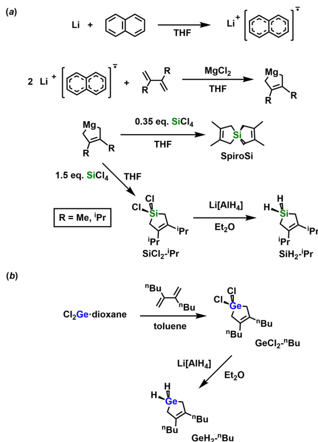
Scheme 1 (a) Synthesis of silaspiro-[4.4]-2,3,7,8-tetramethyl-2,7-nona-diene (SpiroSi) and 1,1-dihydro-3,4-di-iso-propylsilacyclopent-3-ene ( \text{SiH}_2\text{-iPr} ); (b) synthesis of 1,1-dichloro-3,4-dibutylgermacyclopent-3-ene \text{GeCl}_2\text{-}^n\text{Bu} and 1,1-dihydro-3,4-dibutylgermacyclopent-3-ene \text{GeH}_2\text{-}^n\text{Bu} .
