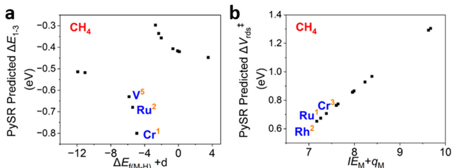
Fig. 6 The scatter plot of (a) PySR-predicted \Delta E_{1-3} of \text{CH}_4 vs. the sum of \Delta E_{1(\text{M-H})} and d and (b) PySR-predicted V_{\text{rds}}^\ddagger of \text{CH}_4 vs. the sum of \text{IE}_\text{M} and q_\text{M} ; dopants with the lowest predicted reaction energies or barriers are labeled in blue and the orange superscript shows the corresponding DFT ranking (taken as the ground truth).
