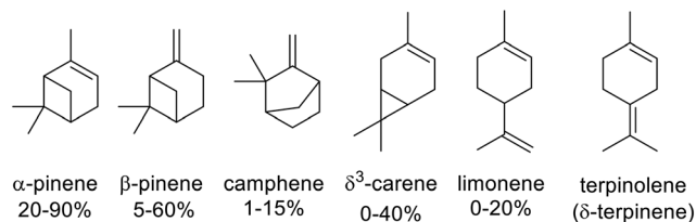
Scheme 1 Turpentine natural components and their variable compositions. 7
