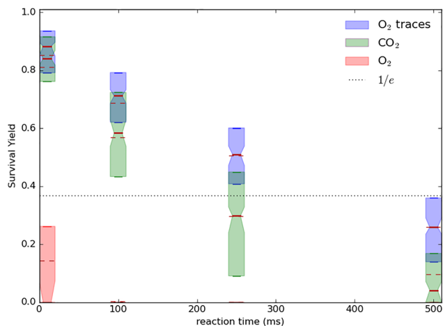
Fig. 9 Evolution of the precursor ion [Mo_6I_{13}]^{2-\bullet} survival yield after variable reaction times in the ion trap filled with various background gas compositions: He with unavoidable traces of O_2 , 0.5% O_2 seeded in helium, 0.5% CO_2 seeded in helium. Boxplot boundaries represent the first and 3 quartiles; thick continuous and thin dashed red lines show the respective positions of the median and the mean for each reaction time dataset. Notches give impressions of the uncertainty windows estimated via a bootstrap approach. The dotted line corresponds to the 1/e level relevant for mono-exponential decays.
