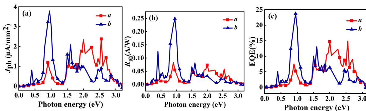
Fig. 11 Linearly polarized light with \theta of 0^\circ generates (a) J_{ph} , (b) R_{ph} , and (c) EQE in the O3 variant when incident in the a and b directions.
