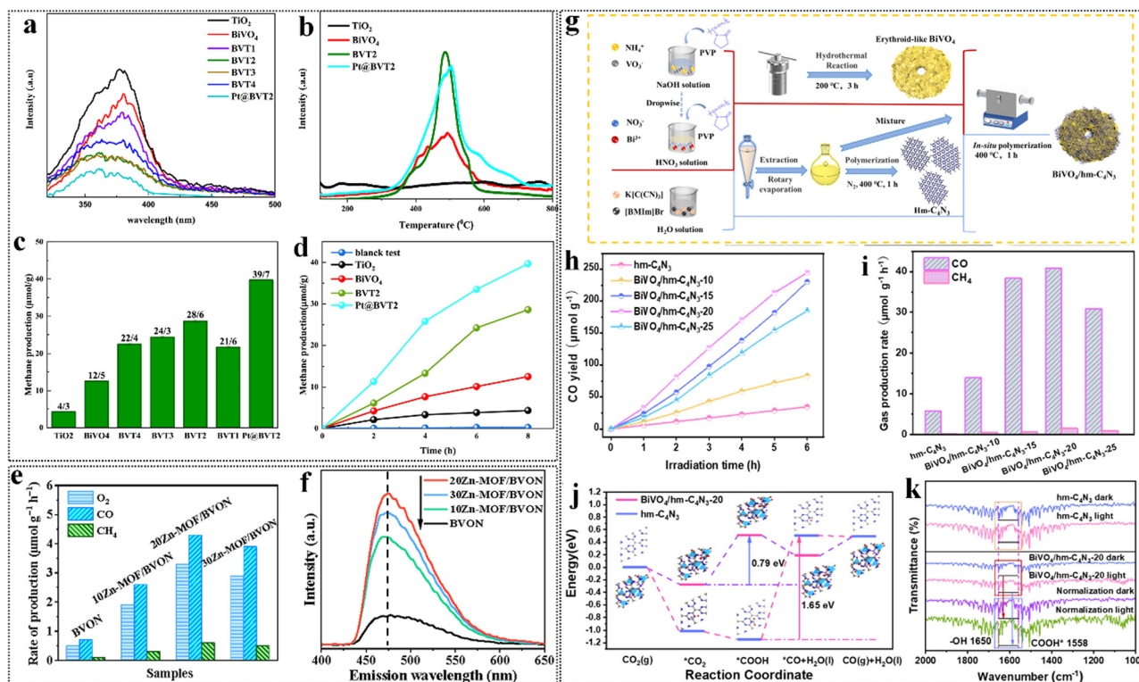
Fig. 6 (a) Photoluminescence spectra of the synthesized photocatalysts. (b) CO 2 -TPD results of TiO 2 , BiVO 4 , BVT 2 and Pt@BVT 2 from 30 to 800 °C. (c) CH 4 yield over different photo-catalysts after 8 h of reaction. (d) CH 4 yield over different photo-catalysts during 8 h of reaction. Reproduced from ref. 135 with permission from Elsevier, copyright 2024. (e) Photocatalytic activities for CO 2 conversion of BVON and xZn-MOF/BVON heterojunctions under visible-light irradiation. (f) FS related to the formed •OH amount. Reproduced from ref. 136 with permission from Elsevier, copyright 2022. (g) Illustration for the preparation of erythroid-like BiVO 4 /hm-C 4 N 3 hybrids. (h) and (i) Time evolutions of CO and average gas production rates over different catalysts. (j) The free energy diagrams of CO 2 reduction to CO for hm-C 4 N 3 (blue line) and BiVO 4 /hm-C 4 N 3 composite (red line) based on DFT calculation. (k) In situ DRIFTS spectra of CO 2 photoconversion over different samples. Reproduced from ref. 137 with permission from Elsevier, copyright 2021.
