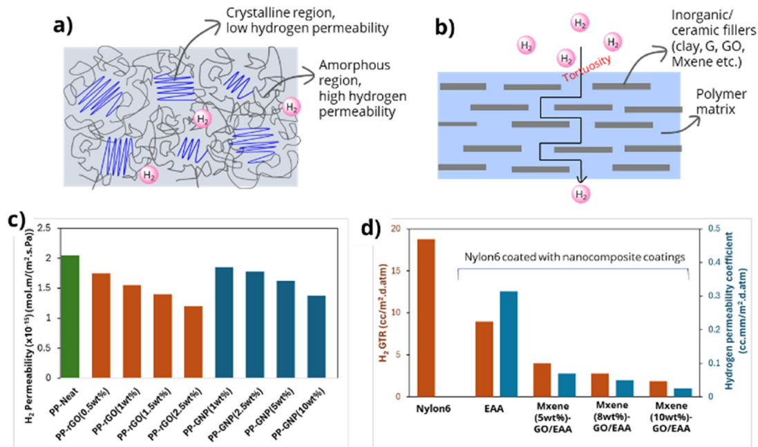
Fig. 14 Hydrogen permeability of (a) a semi-crystalline polymer and (b) a polymer nanocomposite by improving tortuosity. Hydrogen permeability results of (c) PP nanocomposite with rGO and GNP, 80a and (d) nanocomposite of EAA with GO and MXene. 82
