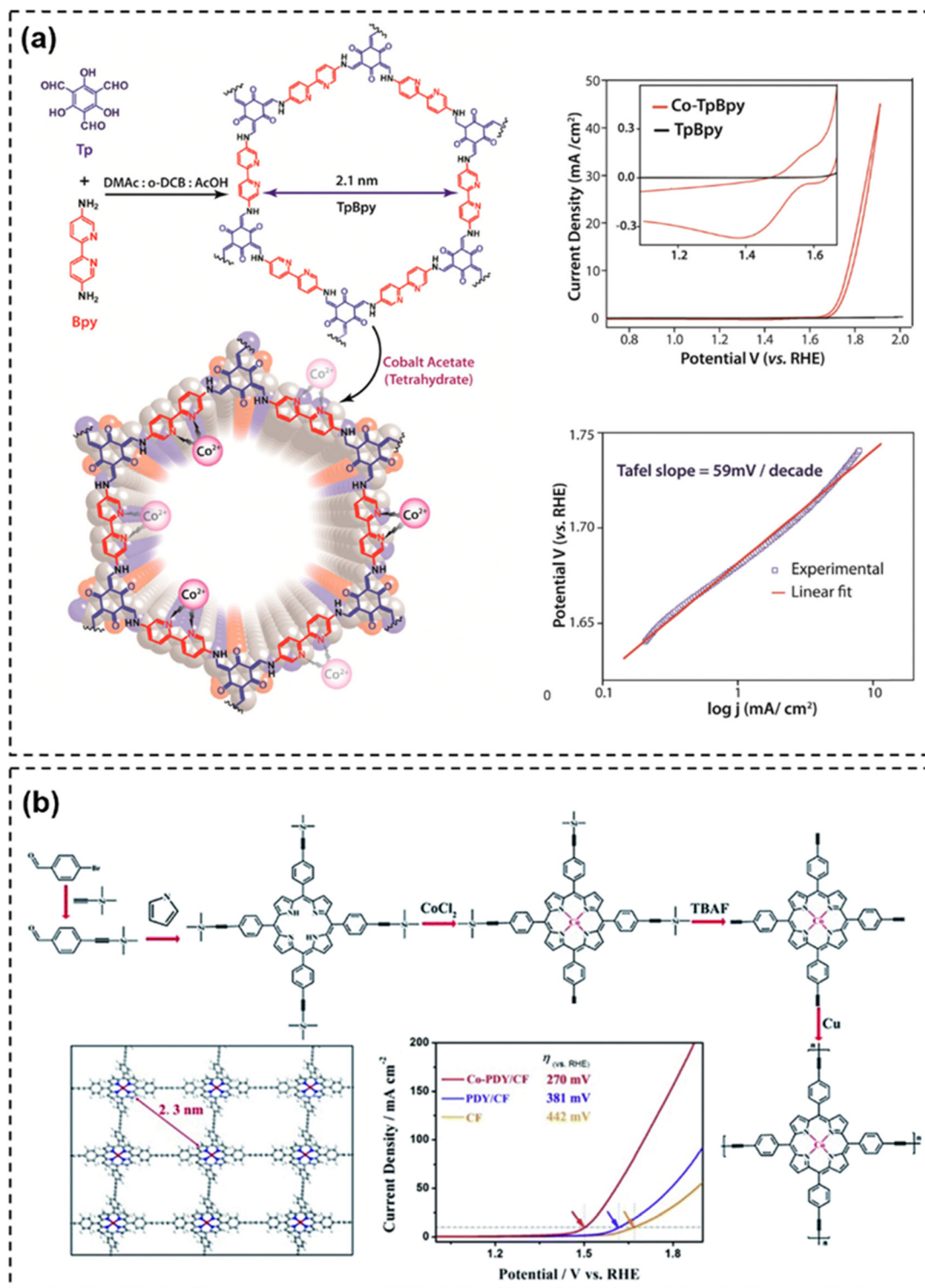
Fig. 12 Active site designed COF-based OER electrocatalysts: Schematic routes to synthesize (a) Co-TpBpy via proton tautomerized Schiff base condensation and \text{Co}^{2+} impregnation with cyclic voltammogram and Tafel plot in a phosphate buffer at pH = 7.0 182 and (b) Co-PDY with LSV curves. 183 Reproduced with permissions from ref. 182 and 183, Copyright 2016 and 2019, with permission from the Royal Society of Chemistry.
