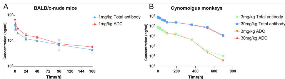
Fig. 5 Pharmacokinetics of JSKN003 in BALB/c-nude mice and cynomolgus monkeys. (A) and (B) Pharmacokinetic profile of JSKN003 in BALB/c-nude mice (A) and cynomolgus monkeys (B). Each treatment group included 5 mice.
