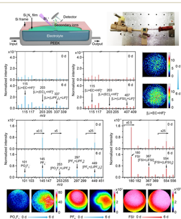
Fig. 12 Schematic illustration and photograph of the ultrahigh-vacuum compatible microfluidic device, and representative in situ liquid ToF-SIMS spectra in the positive and negative ion modes of the LiPF 6 - and LiFSI-based electrolytes before and after high-temperature calendar aging for 6 d (144 h), highlighting the signals of ions related to hydrolysis and showing their intensity evolution. Reprinted with permission from ref. 119. Copyright (2025) Wiley-VCH.
