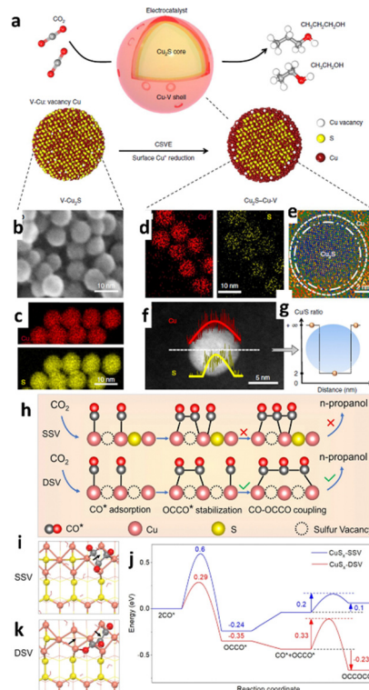
Fig. 11 Catalyst design and structural characterization. (a) Schematic illustration of \text{Cu}_2\text{S} – \text{Cu} – \text{V} CSVE electrocatalyst design for production of multi-carbon alcohols by \text{CO}_2 reduction. (b) and (c) TEM (b) and EDS (c) mapping of the original \text{V} – \text{Cu}_2\text{S} nanoparticles, showing the uniform size and the homogeneous distribution of \text{Cu} and \text{S} . (d)–(g) EDS mapping (d), high-resolution TEM (e), EDS line scan (f) and the ratio of \text{Cu}/\text{S} concentration (g) of the reduced CSVE nanocatalysts after electrochemical reduction, showing the removal of \text{S} from the nanoparticle surface. \text{V} – \text{Cu} indicates \text{Cu} with surface vacancies (reproduced with permission from ref. 142, copyright Nature 2018). (h) The mechanism of n -propanol formation on adjacent \text{CuS}_x – \text{SSV} shows the dimerization of \text{CO} – \text{CO} followed by \text{CO} – \text{OCCO} coupling. (i) and (k) Top views of the optimized \text{OCCOCO}^* intermediate configurations on the (100) surface of (i) \text{CuS}_x – \text{SSV} and (k) \text{CuS}_x – \text{DSV} . The arrows indicate the positions of sulfur vacancies. (j) The corresponding energy diagrams of \text{CuS}_x – \text{SSV} (blue curve) and \text{CuS}_x – \text{DSV} (red curve) at 0 V vs. RHE. The pink, yellow, grey, and red spheres and red wireframe in (h)–(k) represent copper, sulfur, carbon, and oxygen atoms and water molecules, respectively (reproduced with permission from ref. 143, copyright Nature 2021).
