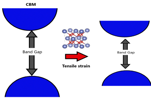
Fig. 7 Bandgap narrowing in SnO 2 under tensile strain due to disorder in SnO 6 octahedra.
