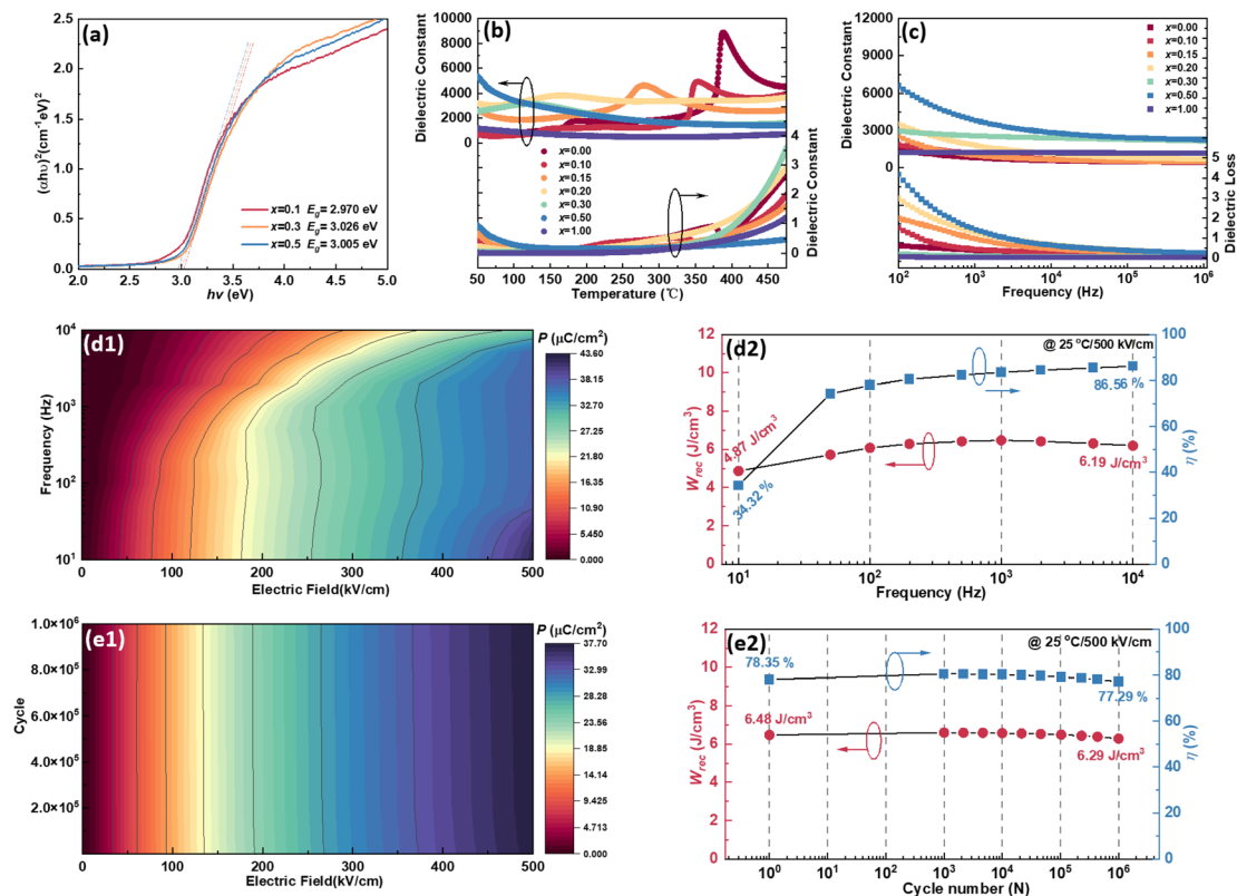
Fig. 6 (a) The fitting results of Fig. S6† according to eqn (15) to obtain the E_g of (1-x)\text{KNN}-x\text{BCZT} with x = 0.1, 0.3 , and 0.5 ; (b) the \epsilon-T curves with \tan \delta-T curves of the (1-x)\text{KNN}-x\text{BCZT} ceramics from 50^\circ\text{C} to 475^\circ\text{C} at 1000\text{ Hz} ; (c) the \epsilon-f curves with the \tan \delta-f curves of the (1-x)\text{KNN}-x\text{BCZT} ceramics from 10^2 to 10^6\text{ Hz} at room temperature; (d1) the mapping to show the variation between polarization and both the applied frequency and the electric field; (d2) the variation between both W_{\text{rec}} and \eta and frequency; (e1) the mapping to show the variation between polarization and both the cycling number and the electric field; (e2) the variation between both W_{\text{rec}} and \eta and the cycling number.
