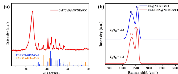
Fig. 1 (a) XRD pattern of CoP/CoN@NCNRs/CC; (b) Raman spectra of CoP/CoN@NCNRs/CC.
