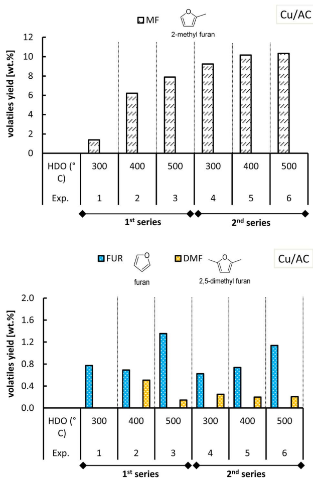
Fig. 12 Yield of MF and other furanics obtained from molten salt hydroxyprolysis of pinewood and subsequent hydrodeoxygenation with Cu/AC. Conditions: 0.4 MPa and hydroxyprolysis at 350 °C.
