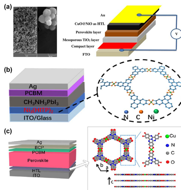
Fig. 6 (a) FE-SEM images of \text{CuO}@/\text{NiO} nanosphere and the corresponding device structure. Reproduced from ref. 51 with permission from Springer Nature, copyright 2020. (b) The device structure and the crystal structure of \text{Ni}_3(\text{HITP})_2 . Reproduced from ref. 54 with permission from Springer Nature, copyright 2022. (c) Device structure of an inverted PSC and the crystal structure of \text{Cu}_3(\text{HHTT})_2 . Reproduced from ref. 53 with permission from American Chemical Society, copyright 2022.
