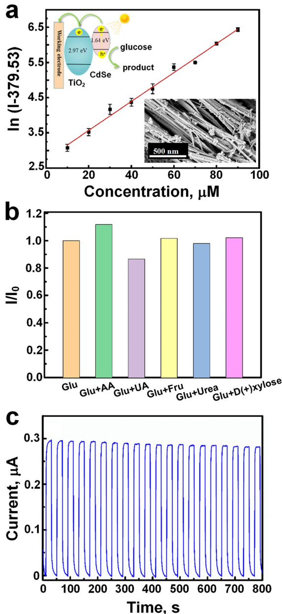
Fig. 12 a) The linearity curve for precise glucose detection between 90 to 10 \mu M concentration. b) Glucose sensing selectivity against different interfering species like ascorbic acid, uric acid, urea, fructose, and D-(+)-xylose. c) Photocurrent stability, and showed no significant change over 800 s (adapted with permission from ref. 130, copyright 2023, American Chemical Society).
