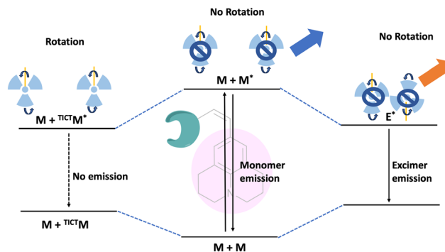
Fig. 1 Modified Jablonski diagram for understanding the fluorogenic response in julolidine-based FMRs, M: monomer, \text{TICTM} : monomer in the twisted intramolecular charge transfer state, \text{M}^* : excited monomer, \text{TICTM}^* : excited monomer in the twisted intramolecular charge transfer state, and \text{E}^* : excimer.
