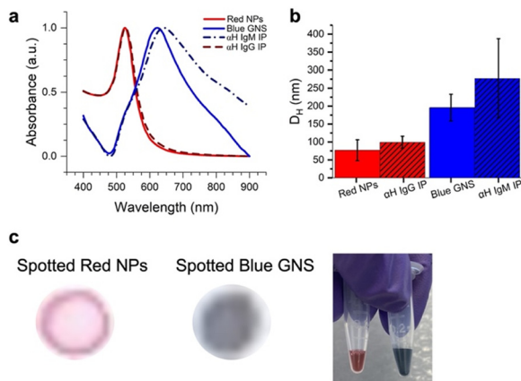
Fig. 3 a) UV-vis spectra of spherical red NPs (red solid line), NP- \alpha IgG (red dashed line), blue GNS (blue solid line) and GNS- \alpha IgM (blue dashed line). b) DLS of NPs (red), NP- \alpha IgG (red hashed), GNS (blue), and GNS- \alpha IgM (blue hashed). c) NP- \alpha IgG and GNS- \alpha IgM spotted on paper and solutions of red NPs and blue GNS.
