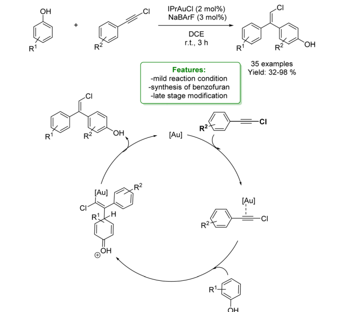
Scheme 63 Au-catalysed alkenylation of phenols with chloroalkyne. 183
