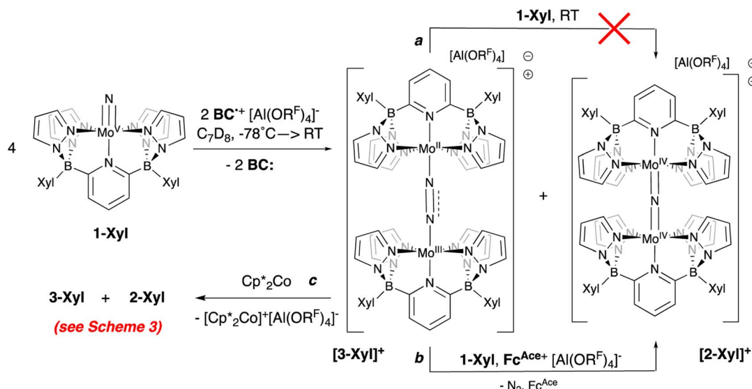
Scheme 5 Reaction of 1-Xyl with 0.5 equivalents of oxidant at -78\text{ }^{\circ}\text{C} and subsequent transformations of the 1 : 1 mixture of [3\text{-Xyl}]^+ : [2\text{-Xyl}]^+ .
