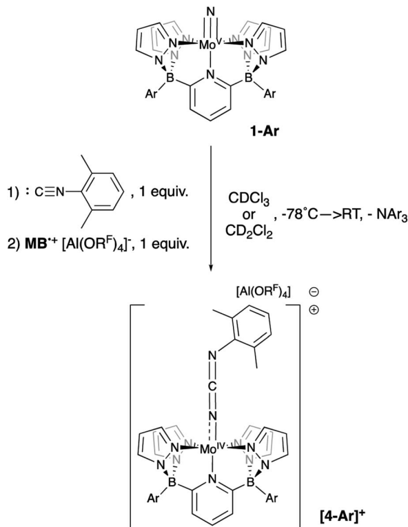
Scheme 6 Reaction of 1-Ar with 1 equivalent of oxidant at -78 °C in the presence of xylal isocyanide.
