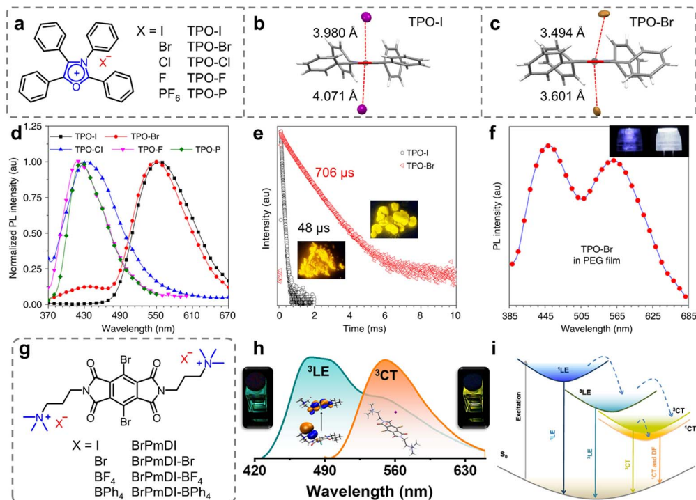
Fig. 1 (a) Chemical structures of TPO-I, TPO-Br, TPO-Cl, TPO-F, and TPO-P. Anion-π interactions with distances for (b) TPO-I and (c) TPO-Br. (d) PL spectra of TPO-I, TPO-Br, TPO-Cl, TPO-F, and TPO-P in the solid state. (e) Time-resolved PL decay of d TPO-I and TPO-Br (insets: photographs of TPO-I and TPO-Br were taken under 365 nm UV irradiation). (f) PL spectra of the PEG film containing TPO-Br (2%, m/m) (insets: photographs of 3D printed lampshades without (left) and with (right) TPO-Br taken under UV-LED lamps). (g) Chemical structures of BrPmDI with different counterions. (h) Normalized PL emission spectra at different excitation wavelengths of 370 nm (cyan line) and 470 nm (orange line) showing the contribution both LE and CT emissions. (i) Jablonski diagram showing various emission processes possible from the LE state of the PmDI core and anion-π-induced CT states. Reproduced with permission from (a–f) ref. 80 (copyright 2018, Springer Nature) and (g–i) ref. 84 (copyright 2022, American Chemical Society).
