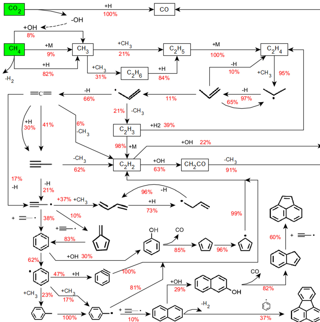
Fig. 8 Integral reaction flow analysis at 1673 K for \tau = 5 s, \text{CH}_4:\text{CO}_2 ratio = 2, and p = 1 bar.
