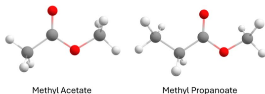
Fig. 1 The structure of the simple esters investigated in this study.
